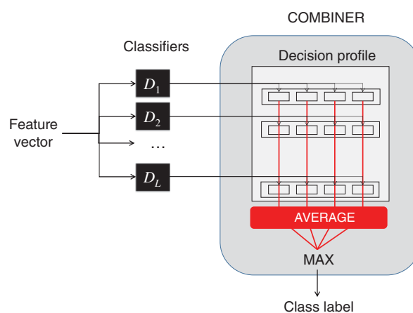
Figure 2: An example of a mean probability combiner. The feature vector for a sample is input to L different classifiers, each of which output a vector of confidence probabilities for each possible class label. These vectors are combined to form the decision profile for the instance which is used to calculate the average support given to each label. The label with the maximum support is then chosen as the prediction. Image reproduced from (Kuncheva, 2014).
