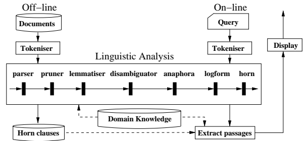
Figure 1. Architecture of the ExtrAns system
