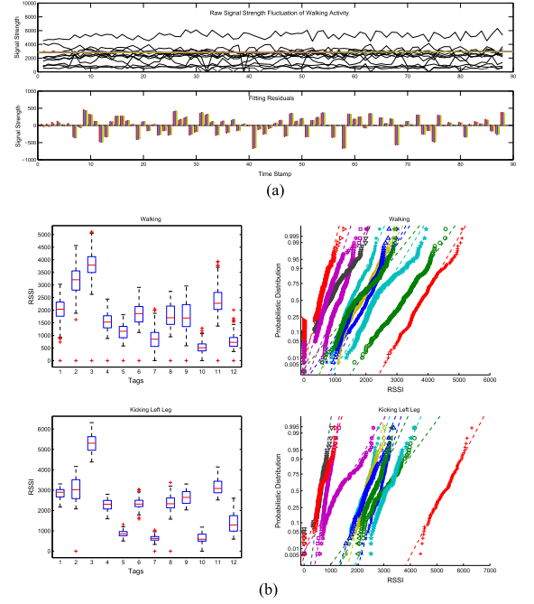
Fig. 2. (a) Signal strength fluctuation of the activity walking and its corresponding linear/quadratic/cubic/polynomial fittings and residuals. (b) The signal distribution pattern of activities walking (top) and kicking left leg (bottom).
