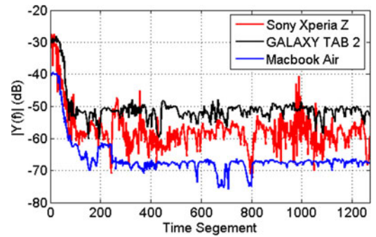
Fig. 4. The sound signal drifts for different mobile devices at different time slots.
