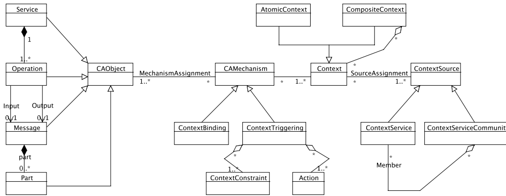
Figure 1. ContextUML metamodel
