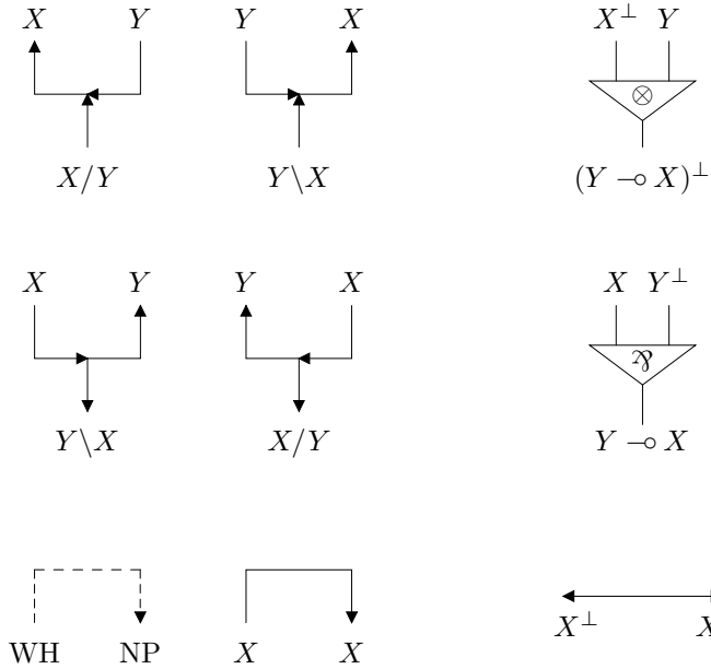
Figure 1. The first two columns list the proof net connectives used here, and the third column provides the corresponding linear logic proof net connective.
