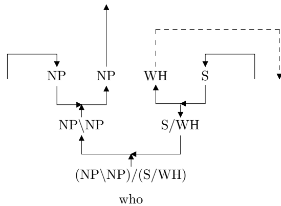
Figure 3. The partial proof net associated with the relative pronoun who .
