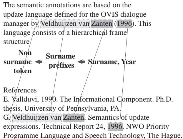
Figure 3: Named entity recognition
