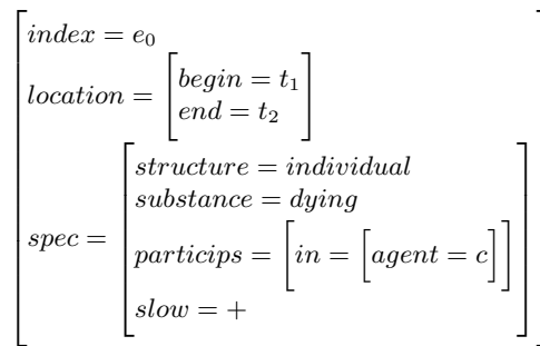
Figure 3: The KBE corresponding to Caesar dies slowly
