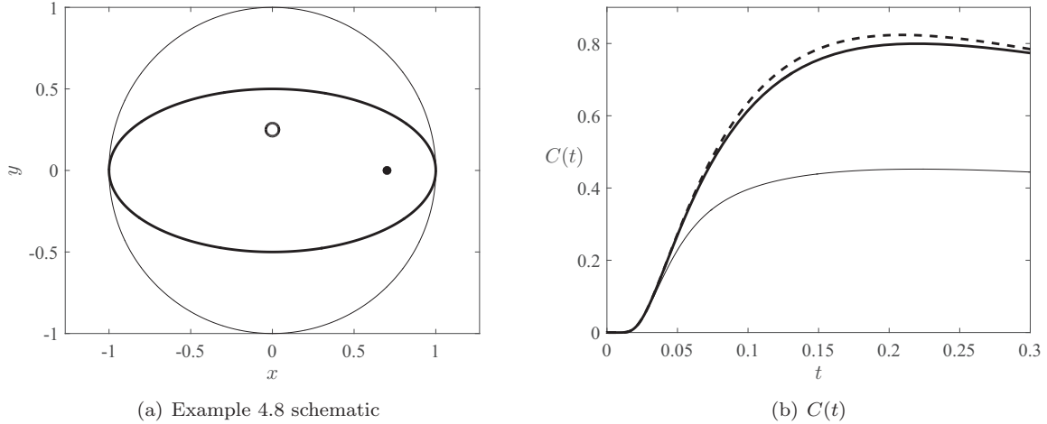
FIG. 11. Schematic and results for Example 4.8. In (a), we show the starting location \mathbf{x}_0 = (0.7, 0) (solid dot) and a circular trap of radius \varepsilon = 0.01 centered at \mathbf{x}_1 = (0, 1/4) . The elliptical (circular) domain is outlined by a heavy (light) solid line. In (b), we show the resulting distribution for C(t) , with the numerical result shown by a heavy solid line and the two-term estimate for the ellipse shown by a heavy dashed line. The light solid line is the two-term estimate for the same trap and starting locations, but with the ellipse replaced by the unit disk.
