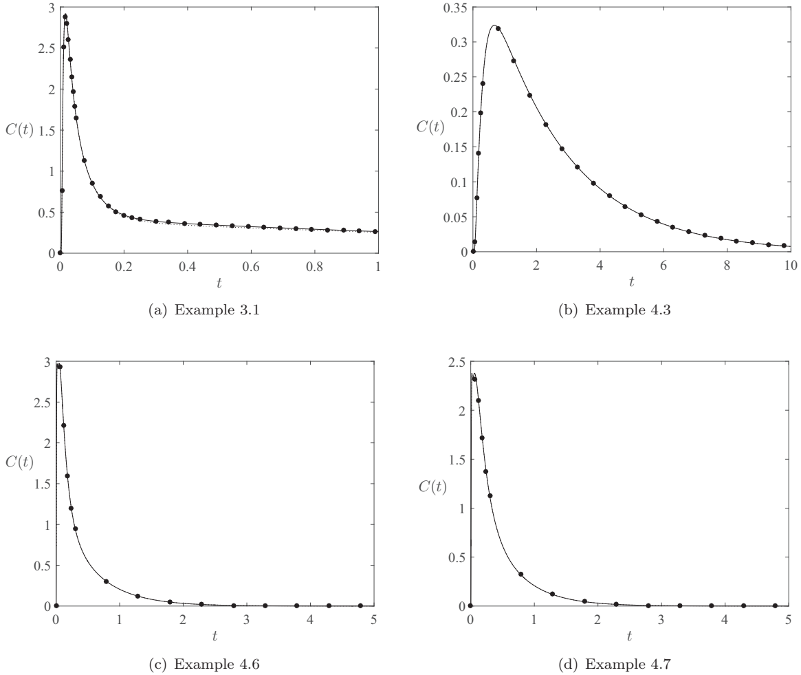
FIG. 12. The full distribution of passage times for the configurations of Examples 3.1, 4.3, 4.6, and 4.7 over large times. Comparison given for full finite-element simulations (solid line) of (1.1), the hybrid-asymptotic method (dashed line), and discrete particle simulations (solid dots). At this scale, the hybrid result is very difficult to distinguish from the exact numerical result.
