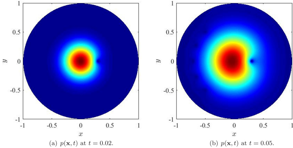
FIG. 9. Snapshots of solution p(\mathbf{x}, t) of (1.1) at (a) t = 0.02 and (b) t = 0.05 for Example 4.6. The times of the two snapshots approximately correspond to the times of the two peaks in C(t) in Fig. 8(b). The first peak occurs as the initial distribution reaches the nearest trap, while the second peak occurs at a later time when the distribution spreads to the second set of five absorbing traps.
