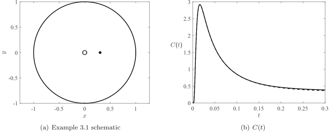
FIG. 2. Schematic and result for Example 3.1. In (a), we show the schematic with one trap of radius \varepsilon = 0.01 centered at the origin (open circle), while the initial starting location for the particle is marked with a solid dot at \mathbf{x}_0 = (0.3, 0) . In (b), we show the exact capture time distribution computed from an eigenfunction solution of (1.1) (solid). A small time estimate obtained from the hybrid method is shown in dashed. Very close agreement is observed when t is small.
