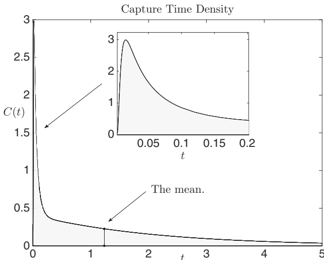
FIG. 1. The full distribution of capture times C(t) for a random walker in the unit disk, starting at (0.3, 0) , and absorption at a circular trap of radius \varepsilon = 0.01 centered at the origin.
