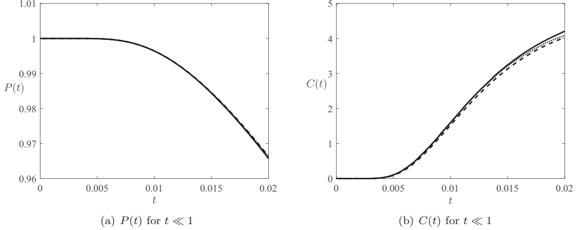
FIG. 4. Results for Examples 4.1 and 4.2. In (a), we show P(t) for M = 3 , \ell = 0.4 , and \varepsilon = 0.01 as numerically computed on the unit disk (solid) and square of side length 2 (dotted). The asymptotic estimate obtained from numerically inverting (4.5) is plotted by a dashed line. The three lines are almost indistinguishable. Details are given in the text. In (b), we show the corresponding plot for C(t) . As expected, the shape and size of the domain have little effect over the small time interval considered, so that (4.5) provides a good estimate for both the circular and square domains.
