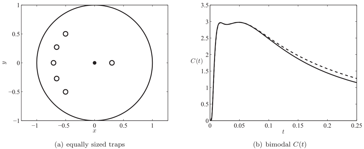
FIG. 8. Schematic and results for Example 4.6. In (a), we show the starting location \mathbf{x}_0 at the origin (solid dot) surrounded by six traps of equal size that form two absorbing sets. The first set consists of the nearest trap centered at (r_1, 0) . The second set is composed of the union of the five traps centered on a ring r_c > r_1 . In (b), we show the resulting bimodal distribution for C(t) . The first peak corresponds to paths straight from \mathbf{x}_0 to (r_1, 0) . The second peak corresponds to direct paths from \mathbf{x}_0 to the second absorbing set. The second absorbing set needs to be larger due to the greater dispersal of paths on the ring r = r_c vs r = r_1 .
