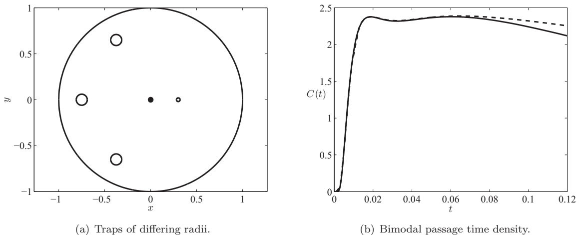
FIG. 10. Schematic and results for Example 4.7. In (a), we show the starting location \mathbf{x}_0 at the origin (solid dot) surrounded by two absorbing sets. The first set consists of the nearest trap centered at (r_1, 0) . The second set is composed of the union of the three traps centered on a ring r_c > r_1 . In (b), we show the resulting bimodal distribution for C(t) . As in Example 4.6, the “wider net” cast by the second absorbing set accommodates the increased dispersal of paths by the time they have reached the ring, r = r_c .
