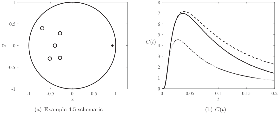
FIG. 7. Schematic and results for Example 4.5. In (a), we show the schematic with \mathbf{x}_0 = (0.92, 0) (solid dot) along with the locations of the five circular traps of radius \varepsilon = 0.01 given by (4.21) (open circles). In (b) we show the full numerical result for C(t) (solid), the two-term asymptotic estimate (dashed), and the boundary-free approximation (dotted). While the two-term estimate better predicts the full result over a longer time interval than does the boundary-free approximation, the interval of agreement is smaller than that seen in Fig. 6 due to the proximity of \mathbf{x}_0 to the boundary.
