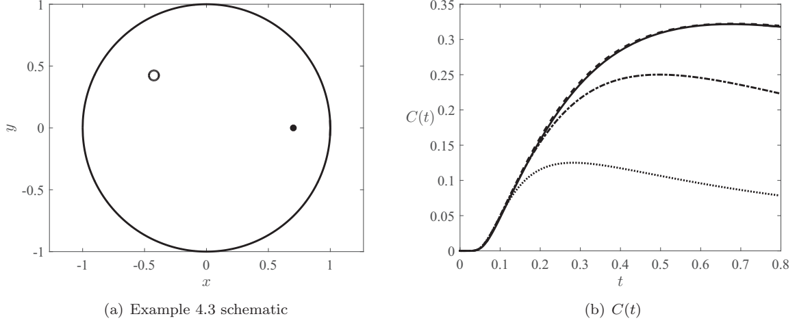
FIG. 5. Schematic and results for Example 4.3. In (a), we show the schematic with one trap of radius \varepsilon = 0.01 centered at \mathbf{x}_1 = r_1(\cos \theta_1, \sin \theta_1) with r_1 = 0.6 and \theta_1 = 3\pi/4 (open circle). The initial walker location (solid dot) is \mathbf{x}_0 = (0.7, 0) . In (b), we show the numerically computed capture time density (solid) along with the boundary-free approximation (dotted), one-term (dash-dotted), and two-term estimates (dashed). The two-term estimate is almost indistinguishable from the numerical solution of (1.1). Note that the two-term estimate is able to accurately predict the location of the mode of C(t) .
