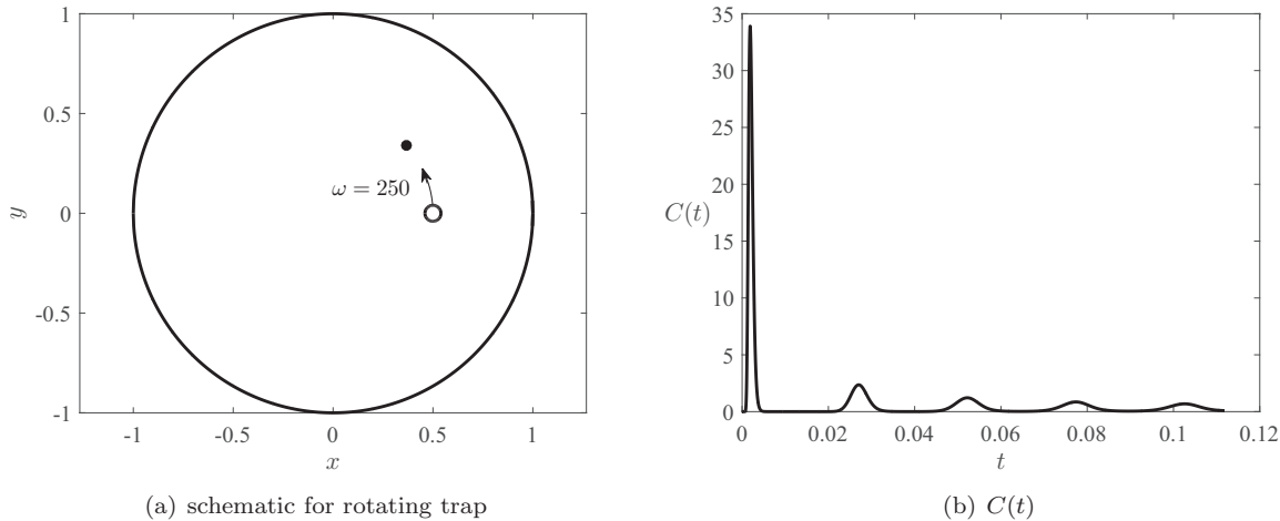
FIG. 13. In (a), we show a schematic of a counterclockwise rotating trap of radius \varepsilon = 1 \times 10^{-5} starting at \mathbf{x}_0 = (0.5, 0) , while the starting location of the particles is at (0.5 \cos(0.5), 0.5 \sin(0.5)) . In (b), we show the capture time density C(t) . The peaks correspond to the capture of particles on each successive sweep of the trap through \mathbf{x}_0 .
