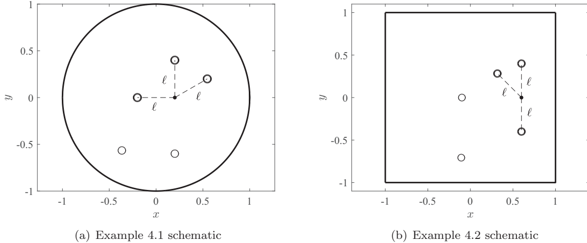
FIG. 3. Schematics of configurations for Examples 4.1 and 4.2. In each figure, the starting location \mathbf{x}_0 for the random walk is marked by a solid dot, while the nearest (farther) traps are indicated by heavy (light) solid circles. In both cases, there are M = 3 nearest traps at a distance \ell = 0.4 from \mathbf{x}_0 . The traps have been enlarged for clarity.
