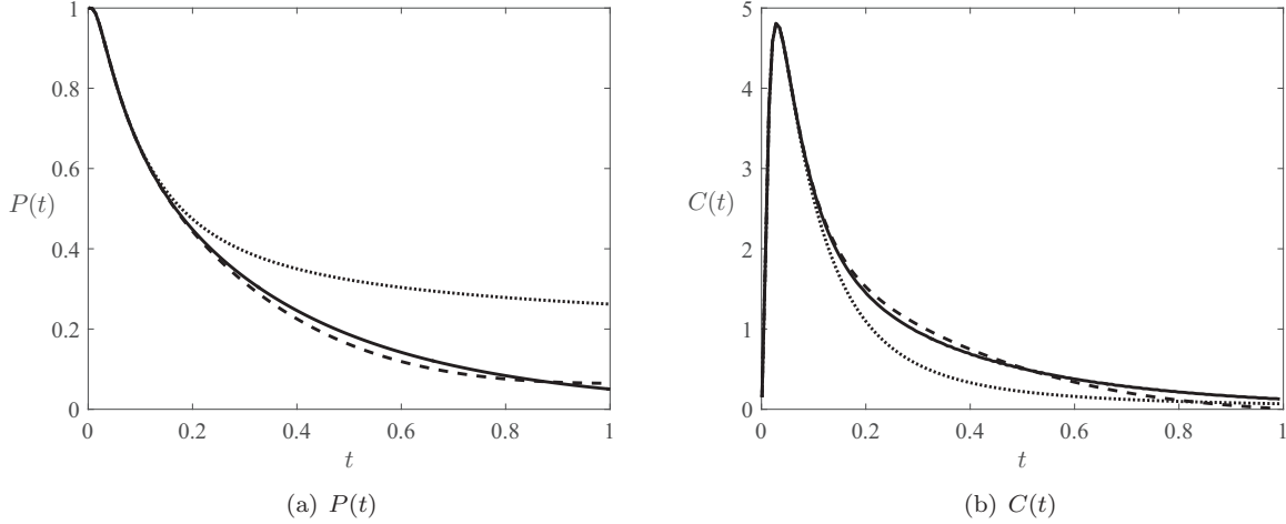
FIG. 6. Results for Example 4.4. In (a), we show the free probability density P(t) for a particle on a unit disk starting a random walk from \mathbf{x}_0 = (0.2, 0) . The locations of the five circular traps of radius \varepsilon = 0.01 are given by (4.6). The full numerical result is shown by a solid line, the two-term asymptotic result by a dashed line, and the boundary-free approximation by a dotted line. In (b), we show the corresponding plots for C(t) . While both the boundary-free and two-term estimates are able to capture the mode of C(t) , the agreement of the two-term estimate persists well past the mode and into the tails of P(t) and C(t) .
